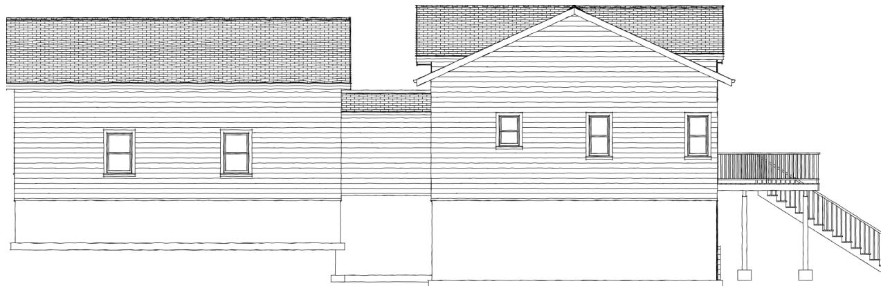
Exterior Elevation Right
